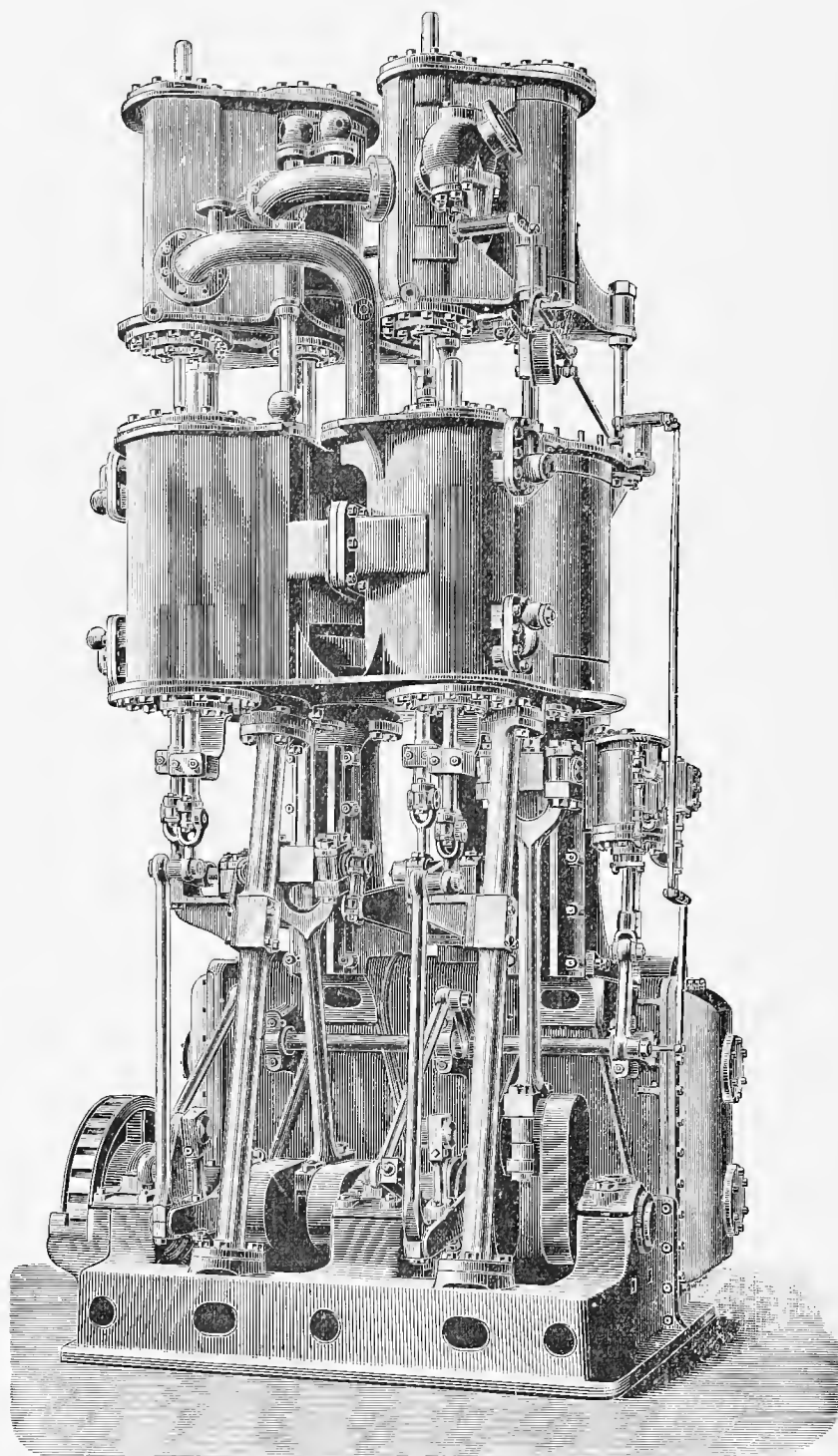
SEE'S QUADRUPLE-EXPANSION ENGINES IN TUG EL TORO.
